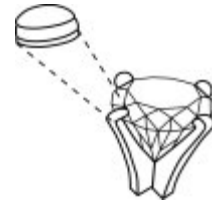
Product ID : REDI.50Y Redi-Prongs Retipping Setting .50 Sold by the dozen only
